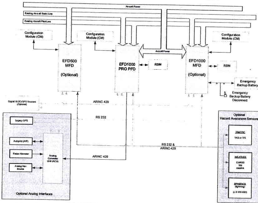
Figure 1 – Block Diagram of the EFD1000 Pro PFD, EFD1000MFD and EFD500MFD System with Optional Interfaces. NOTE: The EA100 (shown in Figure 2) provides pitch and roll data to the autopilot. The ASPEN GTWY (shown in Figure 2) provides communication between the EFD100/500 MFD and certain wireless portable devices. See Table 1 Installed Equipment Configurations.
