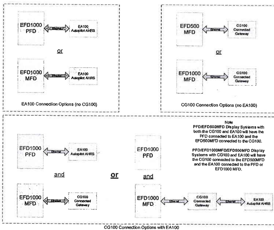
Figure 2- Block Diagram of CG100 and EA100 options. See Table 1 for the configuration of this aircraft.
