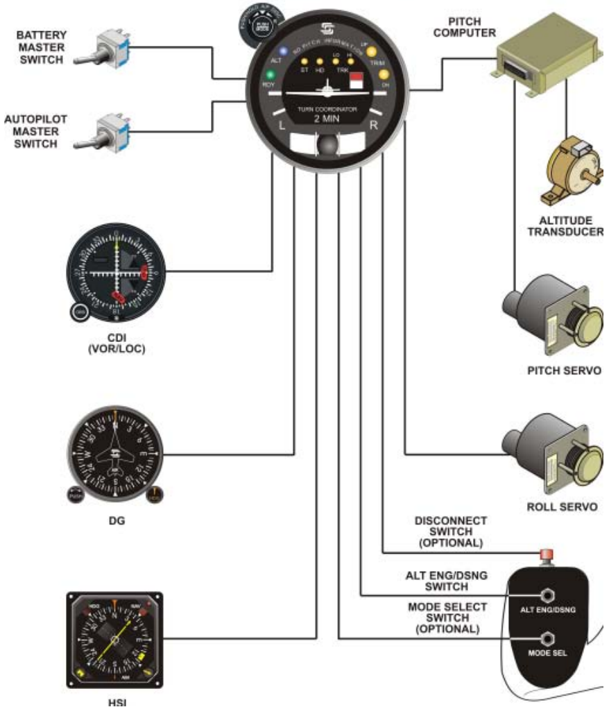
Fig. 1-2. System Thirty Block Diagram
